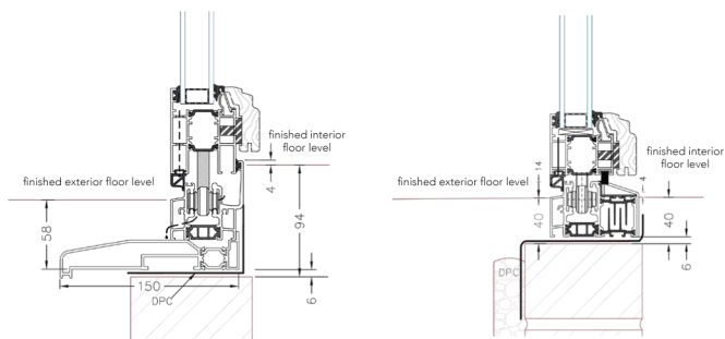
Weathered track on sill
