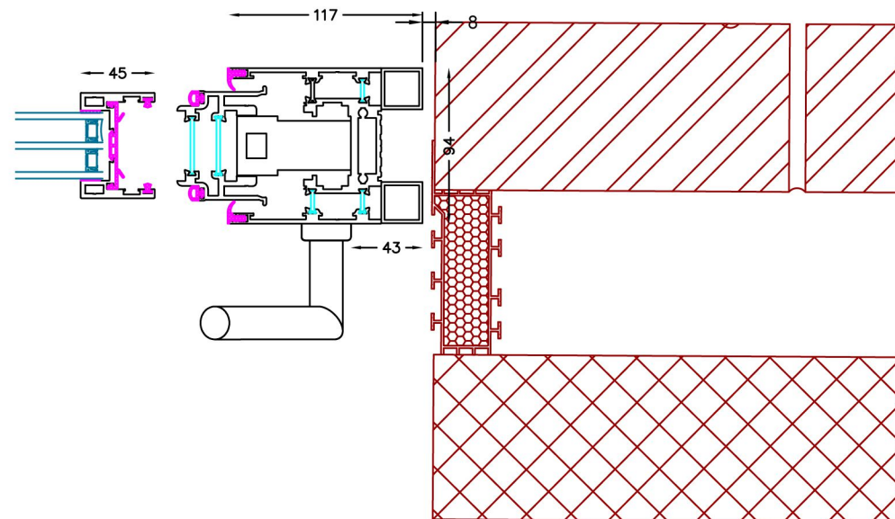
Opening Jamb in Opening Position
