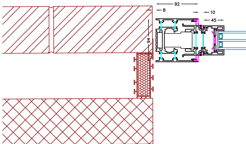
Fixed Jamb in Opening Position
