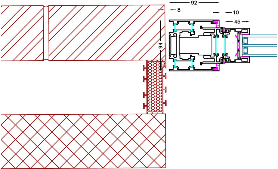
Fixed Jamb in Closed Position
