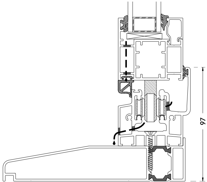
Option 3, Open Out Weathered track on 155mm Thermally Broken Sill
