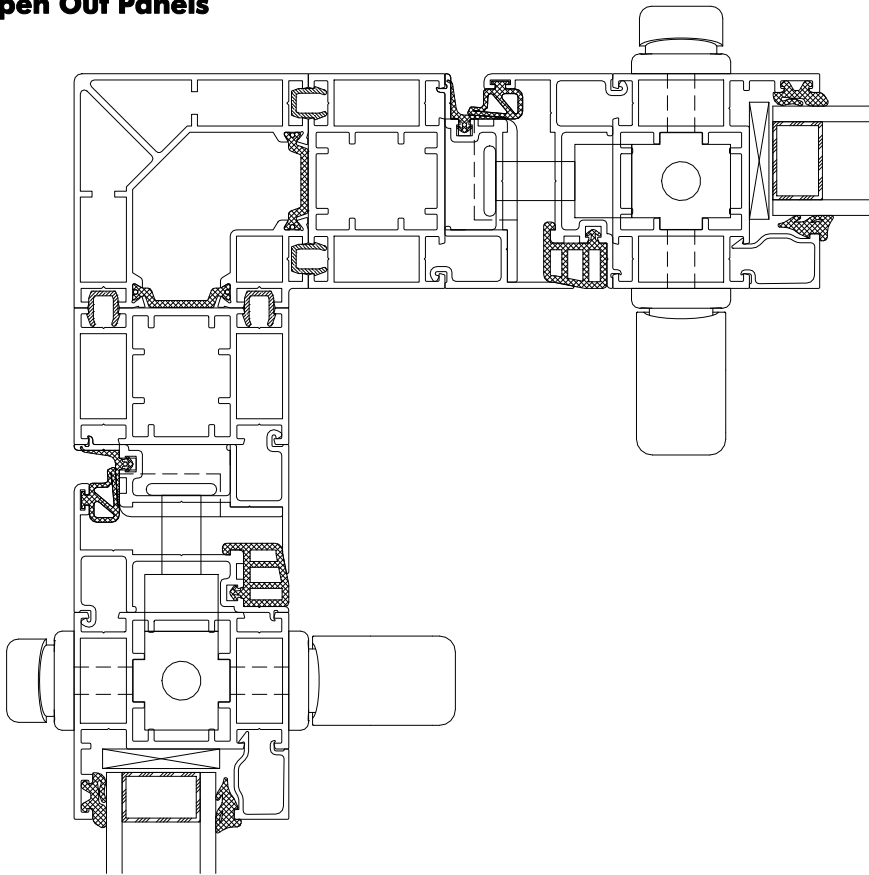
Fixed 90° Post with Open Out Panels
