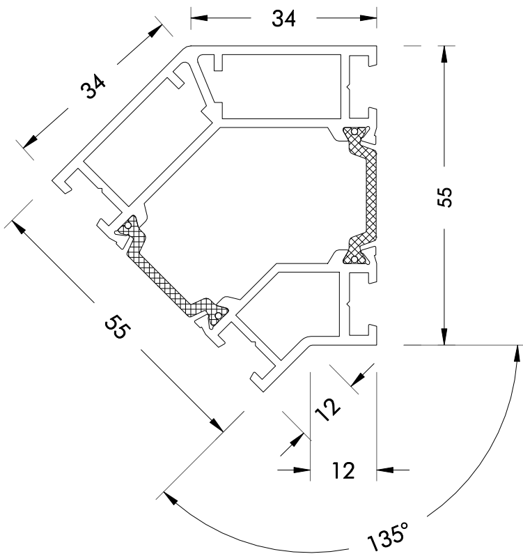
135° Post
