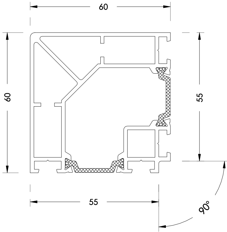
90° Post
