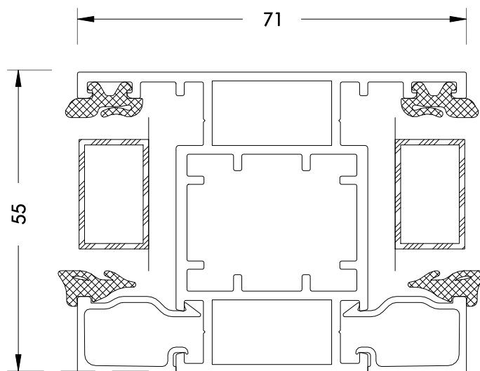
Transom / Mullion
